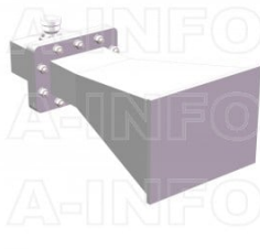
LB-340-10-C-7/16FSPO Standard Gain Horn Antenna 2.2-3.3GHz 10dB Gain 7/16(DIN) Female
