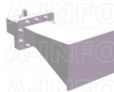
LB-340-10-C-NFSPO Standard Gain Horn Antenna 2.2-3.3GHz 10dB Gain N Type Female
